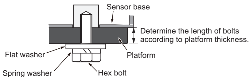
Platform thickness and bolt to use
