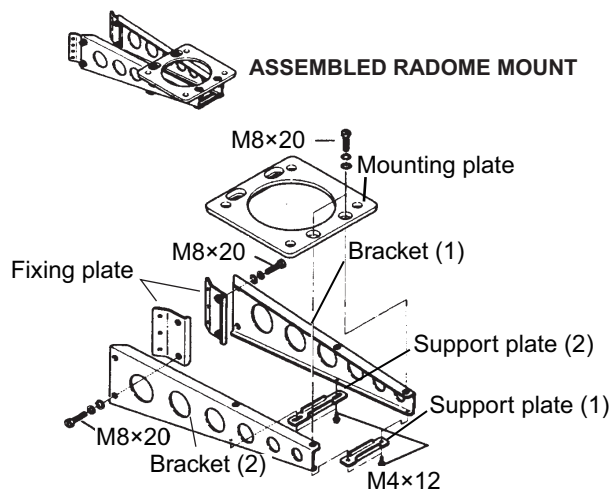
How to assemble the radome mount
