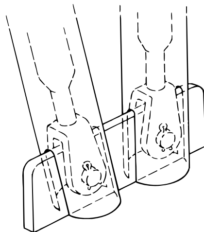
Chain plate wider than tube and tube must be slit.
